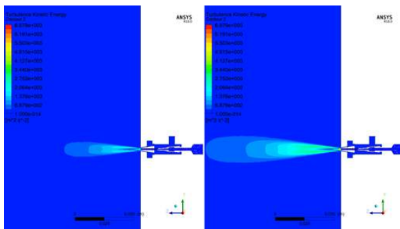
Figure 4. Turbulence kinetic energy contour of air flow.
