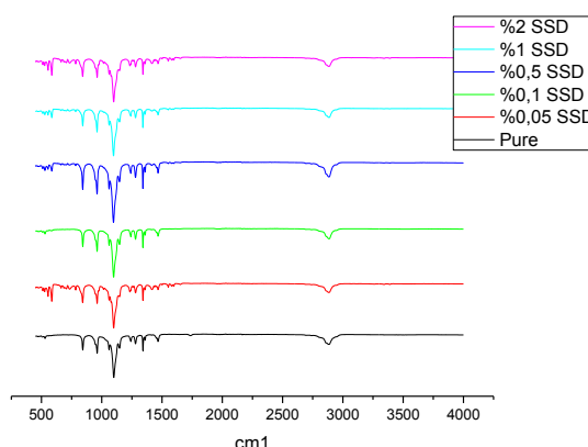
Figure 4. IR Spectra of pure and SSD loaded PEO nanofibers
