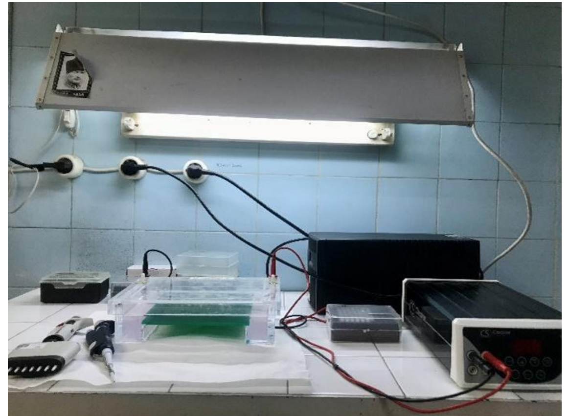
Electrophoresis systems (Clever scientific, MP-250V)
